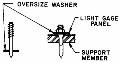
RAMSET TYPE FASTENER
