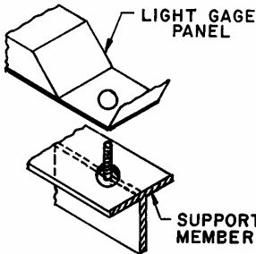
THREADED NELSON TYPE STUDS
